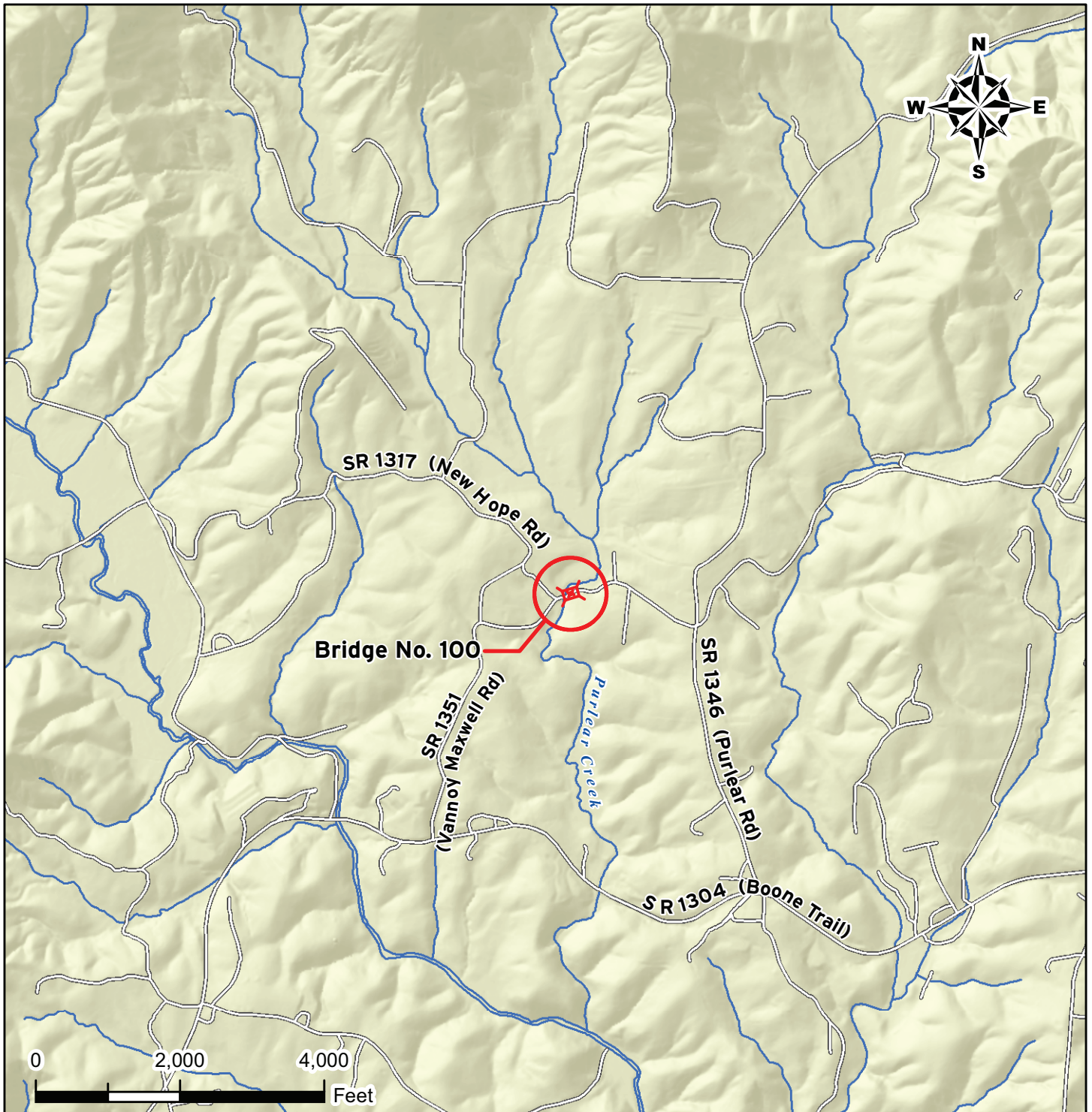
NCDOT Division of Highways Division 11 Low Impact Bridge Replacements Bridge Location Map Bridge No. 100 SR 1317 over Purlear Creek Wilkes County May 2012 Figure 1
